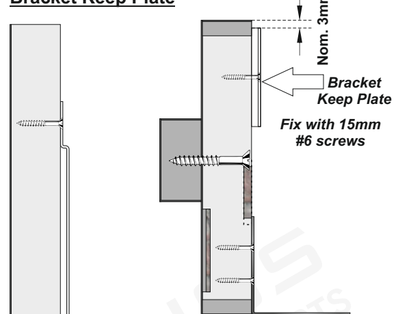
Non-Door Side Bracket Keep Plate
